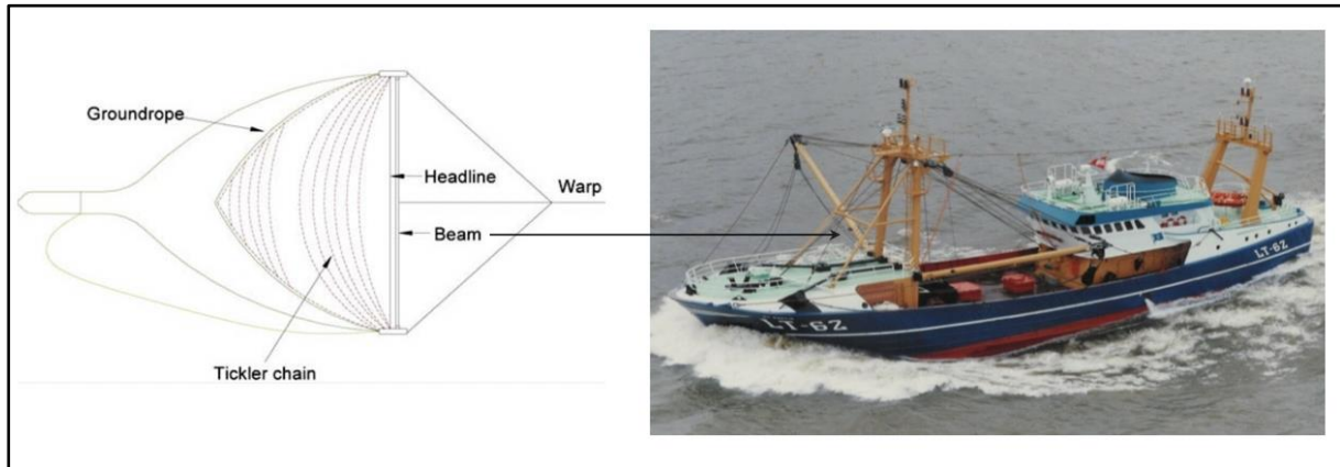
Figure 29: Typical beam trawler vessel and gear diagram (Sources: Visserijnieuws, 2010; FAO, 2005).
