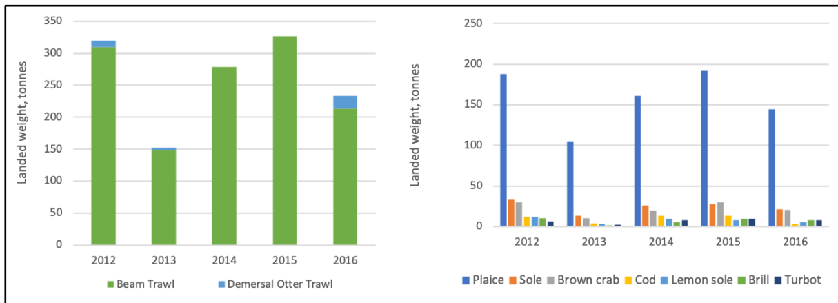
Figure 56: Landed weight of all landings by Belgian registered vessels from ICES rectangles 37F0, 37F1 and 36F1 (array study area) indicating gear type (left) and species (right) (EU DCF database 2019).
