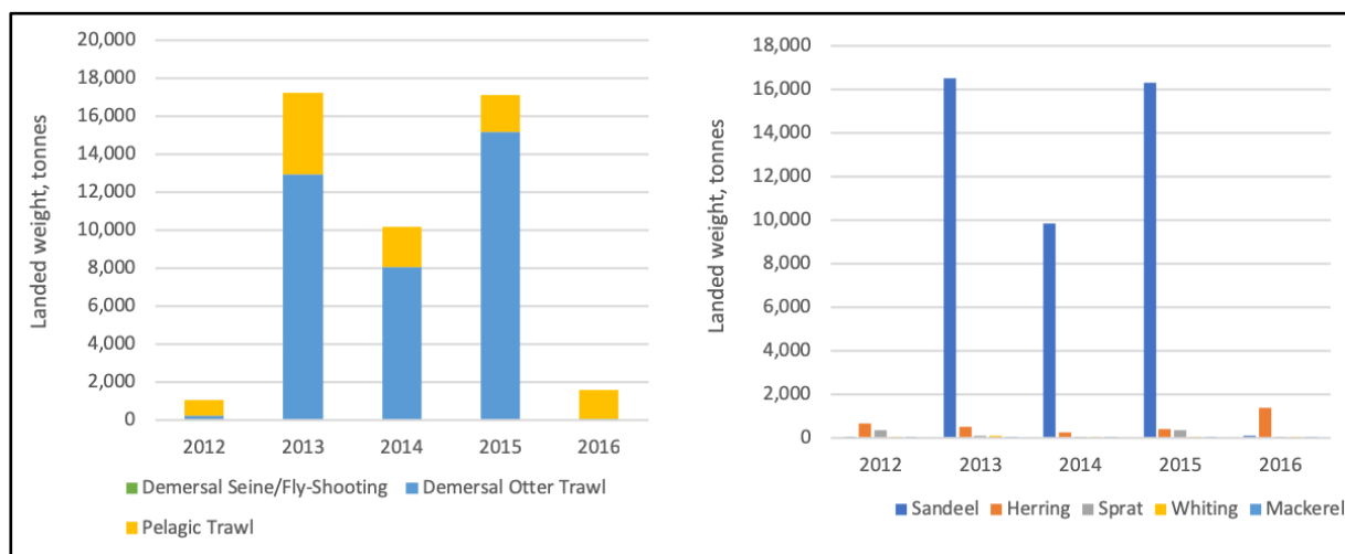
Figure 59: Landed weight of all landings by Danish registered vessels from ICES rectangles 37F0, 37F1 and 36F1 (array study area) indicating gear type (left) and species (right) (EU DCF database 2019).
