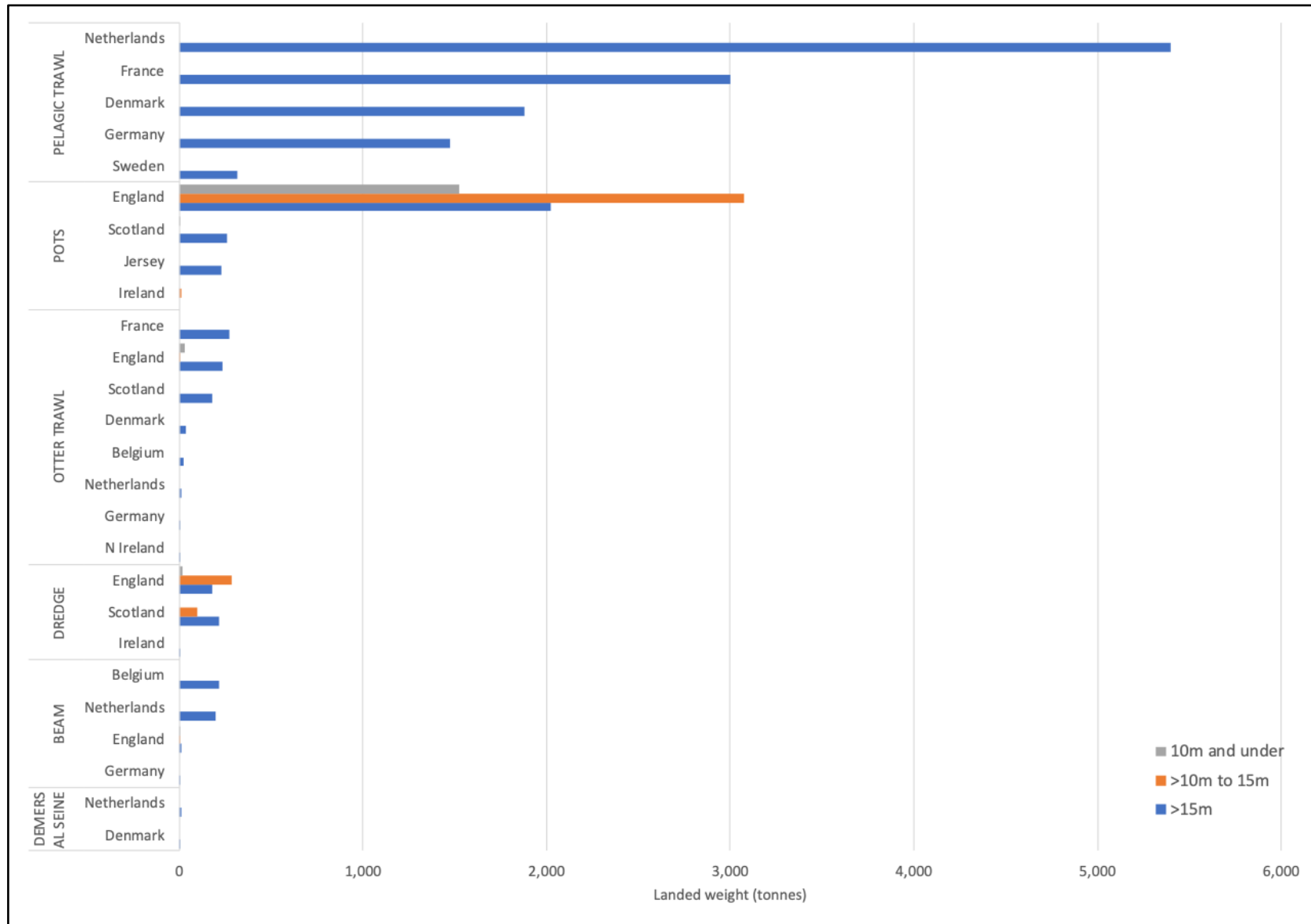
Figure 23: Total landings (tonnes) in 2016, by gear type and vessel nationality for the Hornsea Four commercial fisheries study area (Data source: EU DCF database, 2019).
